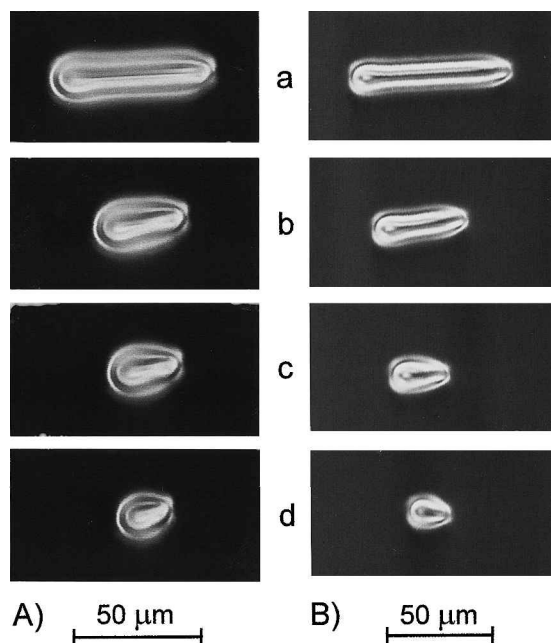
Figure 1. CF-1 fragments observed between crossed polarizers at different voltages. (A) Merck mixture at C = 1.56 , d = 25 \mu\text{m} , f = 100 \text{ Hz} and T = 30^\circ\text{C} : (a) V = V_2 = 6.195 \text{ V} , (b) V = 6.200 \text{ V} , (c) V = 6.300 \text{ V} , (d) V = 6.590 \text{ V} . (B) Roche mixture at C = 1.93 , d = 30 \mu\text{m} , f = 2 \text{ kHz} and T = 50^\circ\text{C} . (a) V = V_2 = 5.192 \text{ V} , (b) V = 5.210 \text{ V} (c) V = 5.220 \text{ V} , (d) V = 5.339 \text{ V} . Photographs 1(a), 1(b), 1(c), ... correspond to curves in figure 2.
