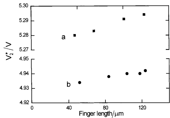
Figure 8. Critical voltage V_2^* as a function of the length of the CF-2 fragment in the Roche mixture at 50^\circ\text{C} . (a) C = 1.93 , d = 30\ \mu\text{m} , f = 2\ \text{kHz} ; (b) C = 1.93 , d = 30\ \mu\text{m} , f = 50\ \text{Hz} .
