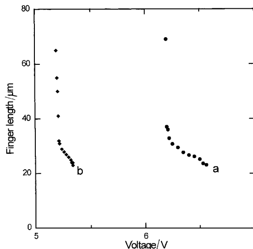
Figure 2. Length L of the CF-1 fragments as a function of the voltage V . L diverges when V \rightarrow V_2 . By convention, velocity v is positive when the finger moves from the rounded tip to the sharp one. See also figure 1. (a) Merck mixture at T = 30^\circ\text{C} and C = 1.56 , d = 25 \mu\text{m} and f = 100 \text{ Hz} ; (b) Roche mixture at T = 50^\circ\text{C} , C = 1.93 , d = 30 \mu\text{m} and f = 2 \text{ kHz} .
