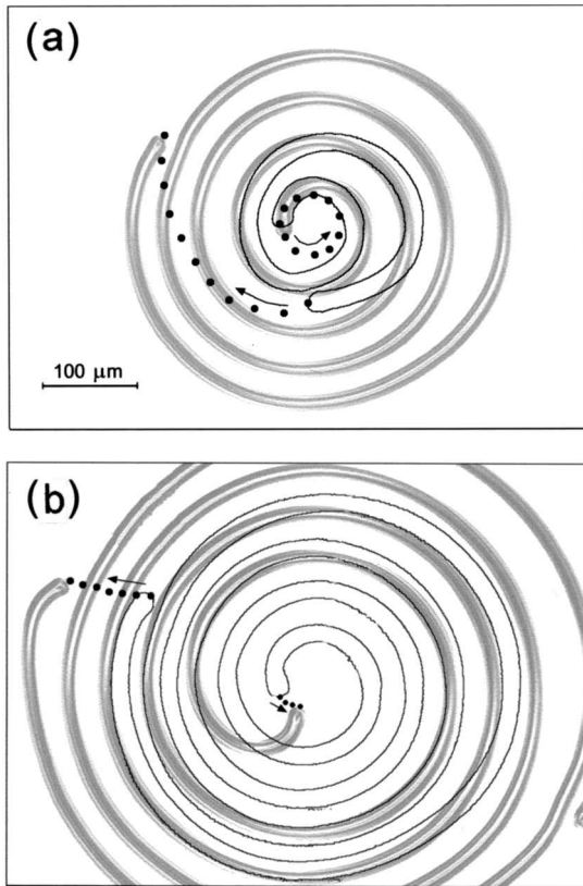
Figure 12. Single spirals in the Roche mixture at C = 1.93 , d = 30 \mu\text{m} , T = 50^\circ\text{C} and different voltages ( V_{2-}^* = 5.264 \text{ V} , V_2 = 5.25 \text{ V} ). (a) V = 5.144 \text{ V} ; the inner tip describes a circle (at angular velocity 73^\circ \text{min}^{-1} ) and the outer tip a logarithmic spiral. Outline t = 0 \text{ min} , shadow sketch t = 10 \text{ min} . (b) V = 5.24 \text{ V} ; both tips describe an open trajectory. Outline t = 0 \text{ min} , shadow sketch t = 9 \text{ min} . Dots on the photographs show the tip trajectories.
