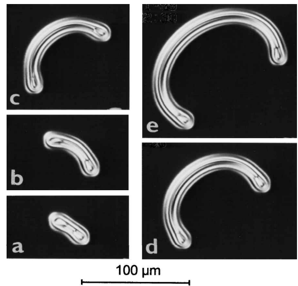
Figure 9. Fragments of a CF-2 observed in the Roche mixture at T = 50^\circ\text{C} , C = 1.93 , d = 30\ \mu\text{m} , f = 2\ \text{kHz} . Crossed polarizers. (a) V = 5.280\ \text{V} , (b) V = 5.283\ \text{V} , (c) V = 5.294\ \text{V} , (d) V = 5.264\ \text{V} , (e) V = 5.266\ \text{V} .
