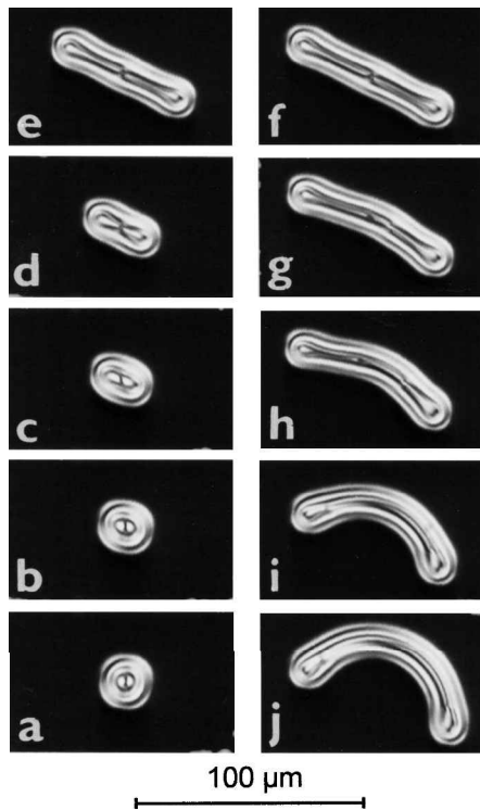
Figure 6. Nucleation and growth of a CF-2 segment by splitting of a cholesteric bubble in the mixture Roche 3421 at 50^\circ\text{C} . C = 1.93 , d = 30\ \mu\text{m} , f = 2\ \text{kHz} . (a) V = 5.06\ \text{V} ; (b) V = 5.03\ \text{V} , t = 0 ; (c) V = 5.03\ \text{V} , t = 10\ \text{s} ; (d) V = 5.03\ \text{V} , t = 14\ \text{s} ; (e) V = 5.03\ \text{V} , t = 27\ \text{s} ; (f) V = V_2^* = 5.25\ \text{V} , t = 76\ \text{s} ; (g) V = 5.25\ \text{V} , t = 155\ \text{s} ; (h) V = 5.25\ \text{V} , t = 176\ \text{s} ; (i) V = 5.25\ \text{V} , t = 219\ \text{s} ; (j) V = 5.25\ \text{V} , t = 280\ \text{s} . Crossed polarizers.
